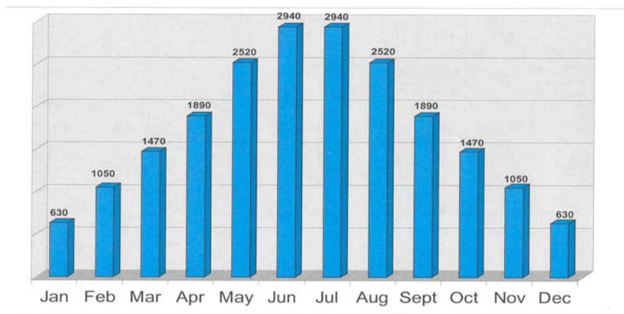
Fig. 43 Monthly Water Amounts for a Mature Date Palm Watering an Area with a 30 ft. diameter. Canopy. Low/Medium Water 21,000 gallons per year.
