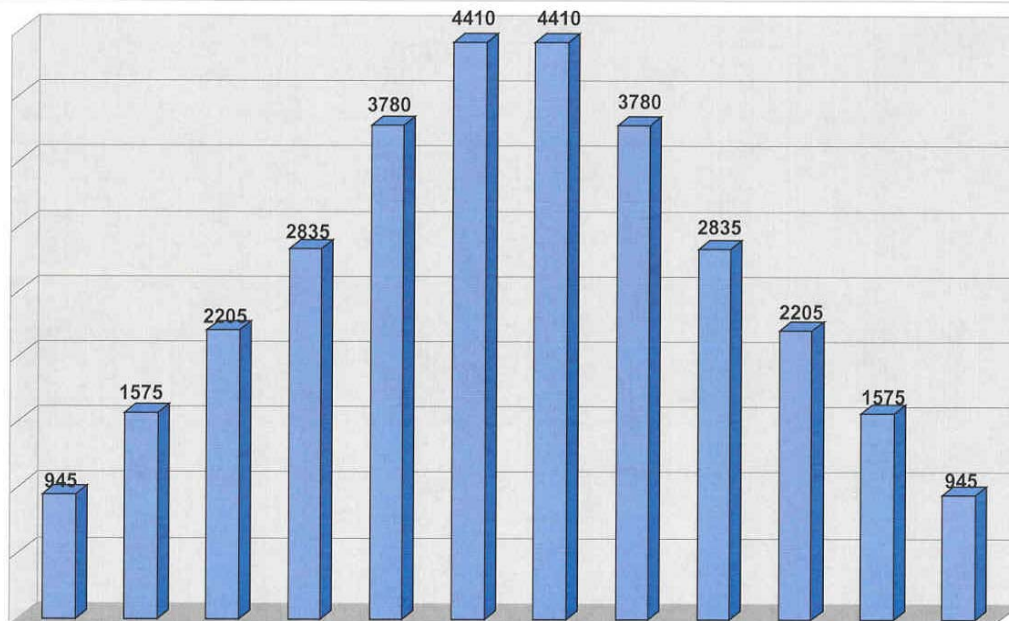
Fig. 44 Monthly water amounts for a mature date palm watering an area with a 30 ft. diameter canopy high median watering with total 31,500 gal/yr.
